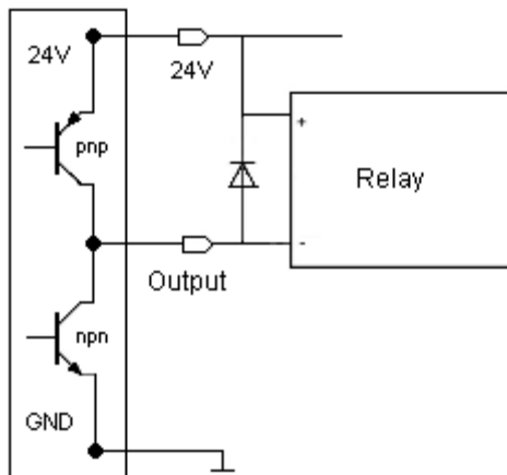
Fig. 5: Connecting output Q1 to relay
