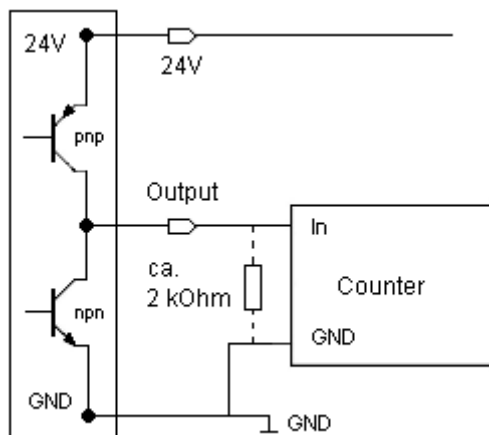
Fig. 6: Connecting output Q2 to counter
