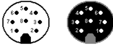
Fig. 4: Pin code: Connection plug / socket
