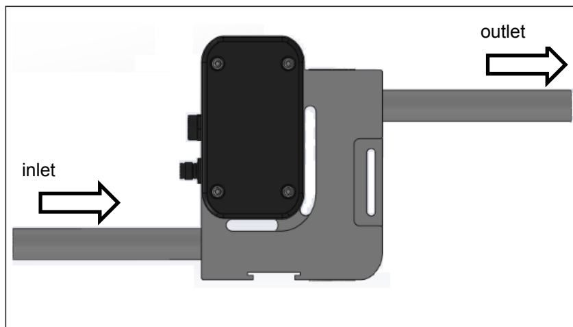
Fig. 2: Installation position of Flowmax 42i
