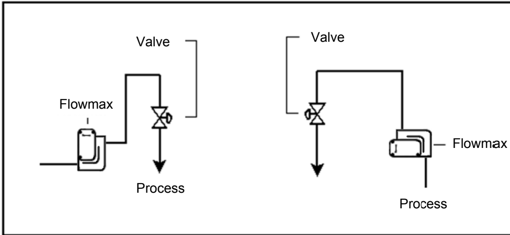
Fig. 4: Mounting possibilities
