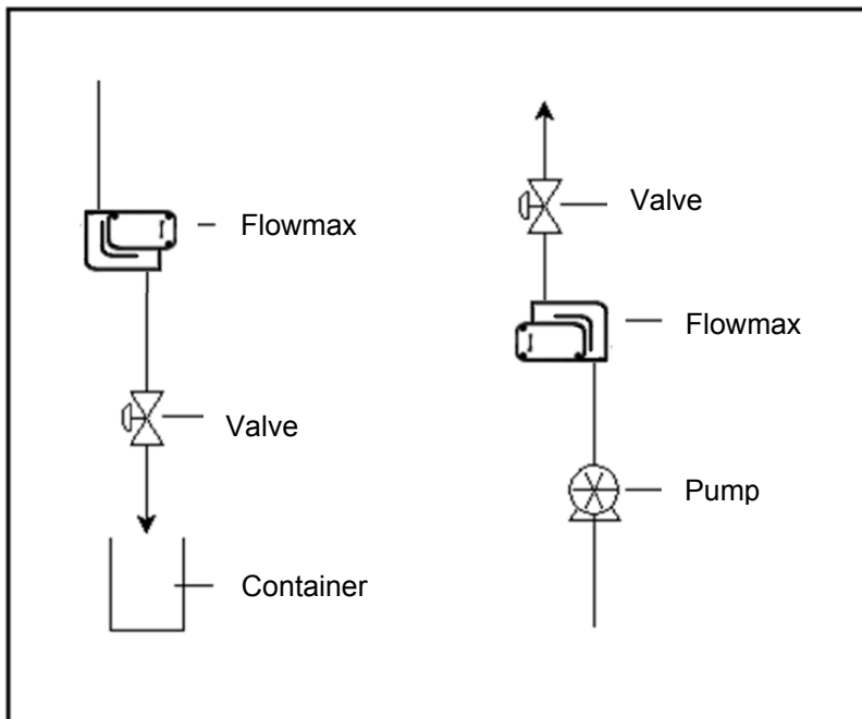
Fig. 3: Mounting examples for Flowmax 42i
