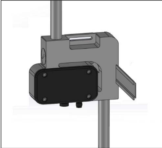
Fig. 6: Flowmax 42i mounted on a DIN rail
