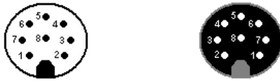
Fig. 8: Pin code: Connection plug / socket for 8-pin version
